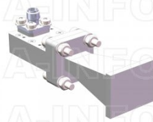
LB-42-10-C-SFSPO Standard Gain Horn Antenna 18-26.5GHz 10dB Gain SMA Female
